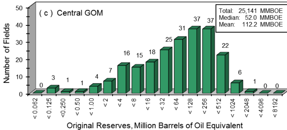
Figure 5. Field-size distribution of oil fields: (a) GOM, 246 fields; (b) Western GOM, 22 fields; (c) Central GOM, 224 fields.
