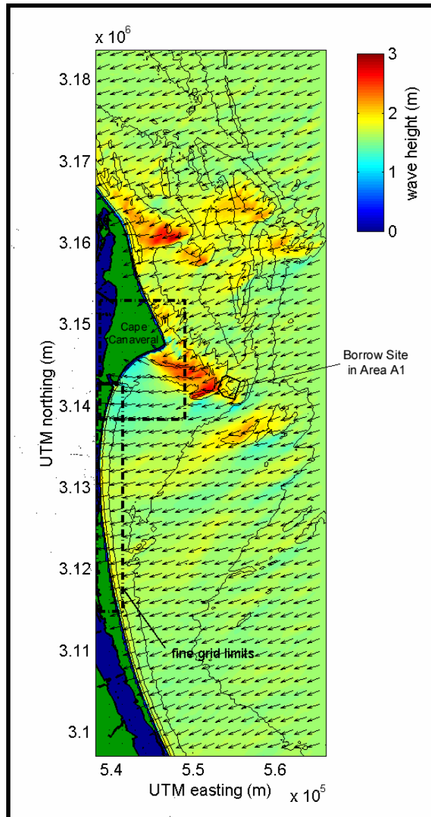
Figure 11. STWAVE output for wave modeling Area A, wave Case 6A ( H_s = 1.6 m, T_{peak} = 14.3 sec, \bar{\tau}_{peak} = 65 deg). Color contours indicate wave height, and vectors show mean direction of wave propagation. Sea floor contours are shown at 5 m intervals.
