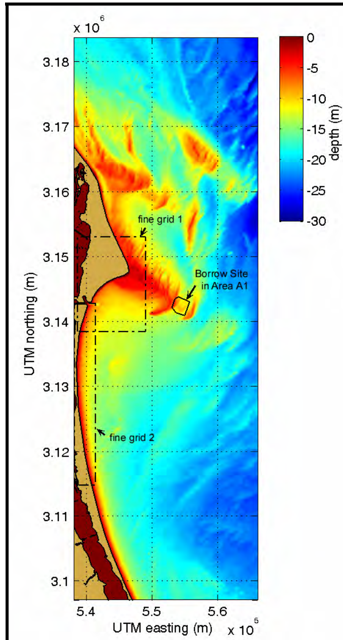
Figure 9. Coarse model grid (200 x 200 m spacing) used for STWAVE simulations offshore Cape Canaveral, FL. Depths are relative to NGVD. Borrow site location is indicated by the solid black line, and fine grid limits are indicated by a dashed line.
