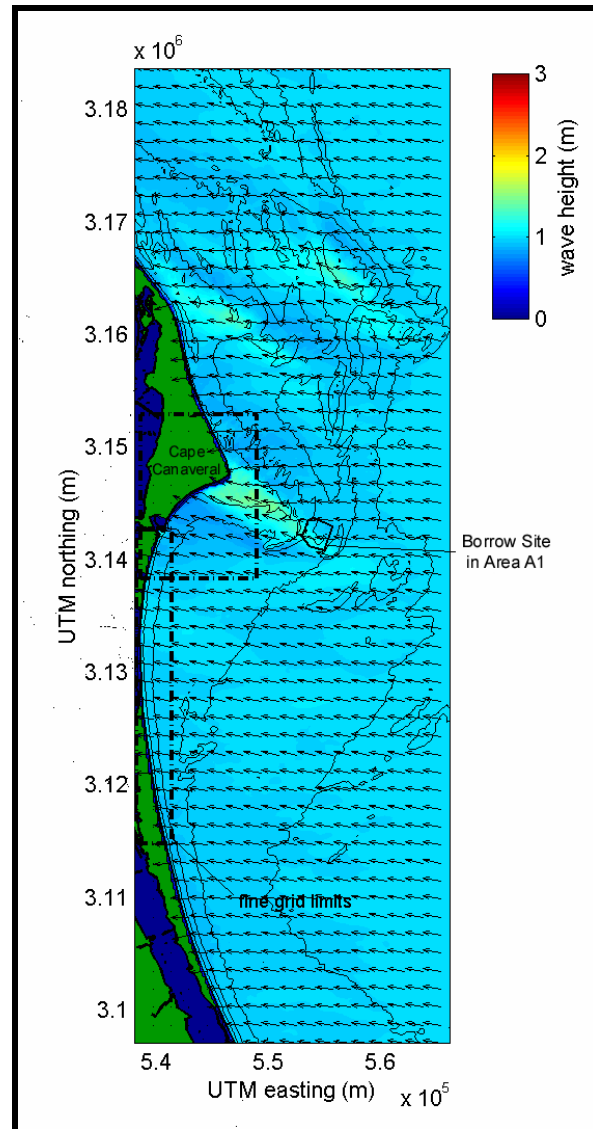
Figure 10. STWAVE output for wave modeling Area A, wave Case 3A ( H_s = 1.0 m, T_{peak} = 7.7 sec, \sim \text{peak } k = 100 deg). Color contours indicate wave height, and vectors show mean direction of wave propagation. Seafloor contours are shown at 5 m intervals.
