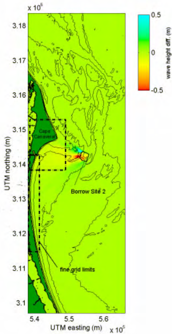
Figure 17. Plot of wave height change between existing and post-dredging ( =H_{post}-H_{pre} ) conditions at borrow site at Canaveral Shoals, ( H_s=1.6 m, T_{peak}=14.3 sec, \theta_{peak}=65 deg).
