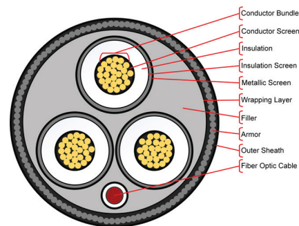
Cable cross-section
