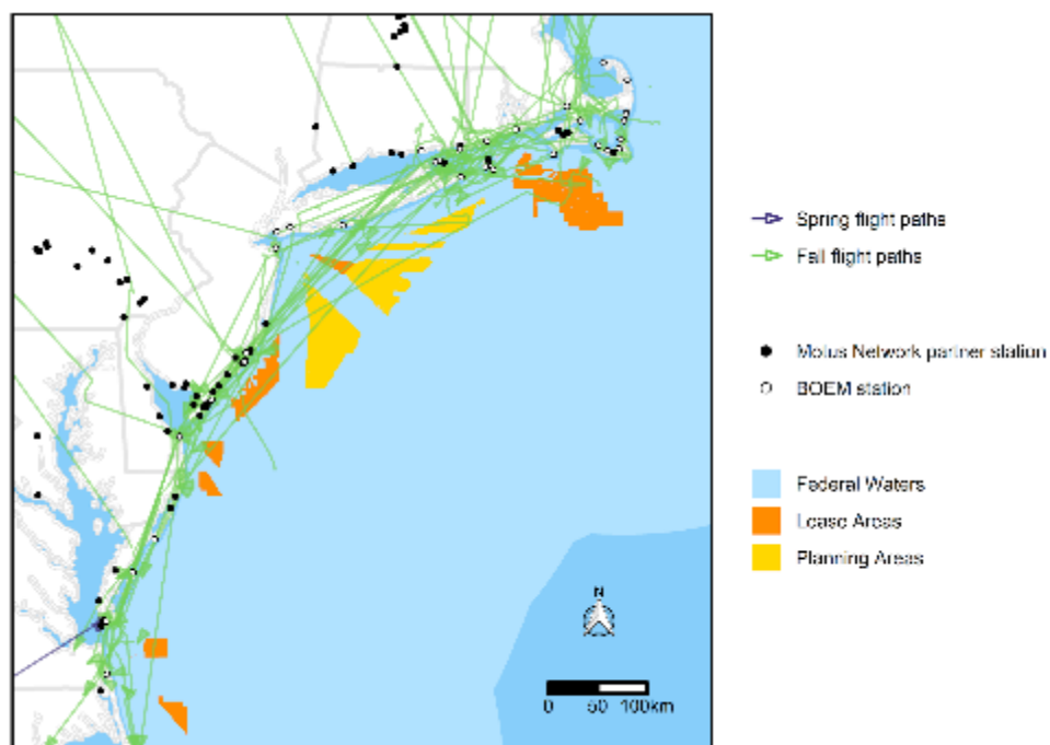
Figure 16. Modeled flight paths of Sanderling crossing the Study Area during spring migration ( n = 1 ) and fall migration ( n = 60 ) in 2015 to 2017.
